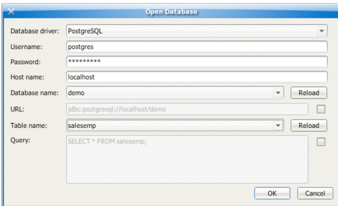
Figure 3. Database query dialog
